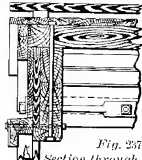
Fig. 2371. Part Section at Door.
